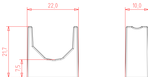
Fixiersockel, Art.Nr. 22-11800-110
